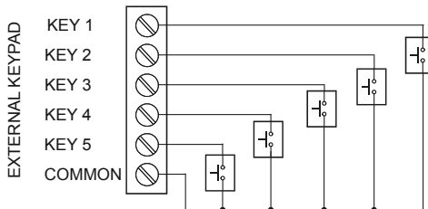
Figure 16. External Keypad Connections
